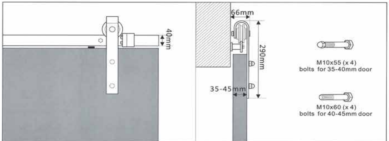
Connection way
